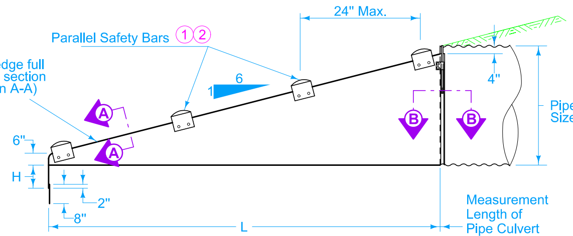
SIDE ELEVATION
