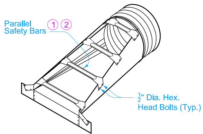
PERSPECTIVE VIEW OF APRON
