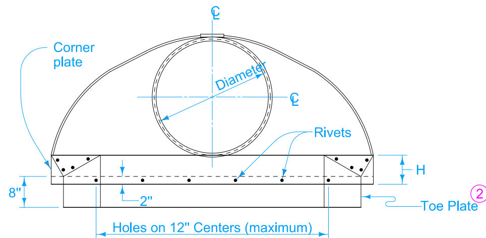
END VIEW
