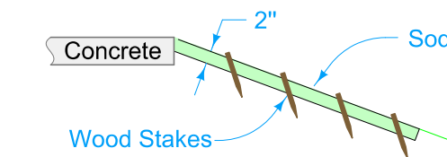
Grade ground surface 2" below the edge of concrete before sod is placed.
