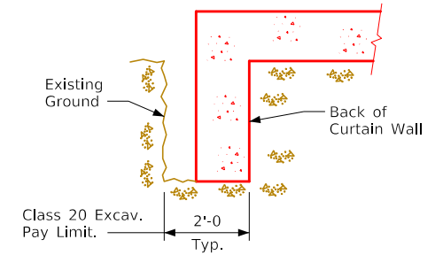
Curtain Wall Class 20 Excavation
