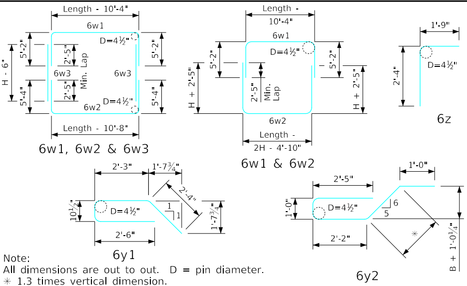
Bent Bar Details
