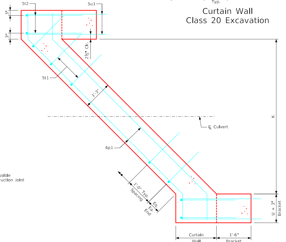
Curtain Wall Detail - Plan View
