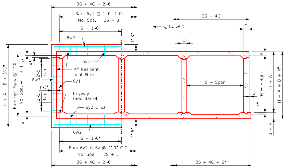
Joint Detail Section thru Barrel
