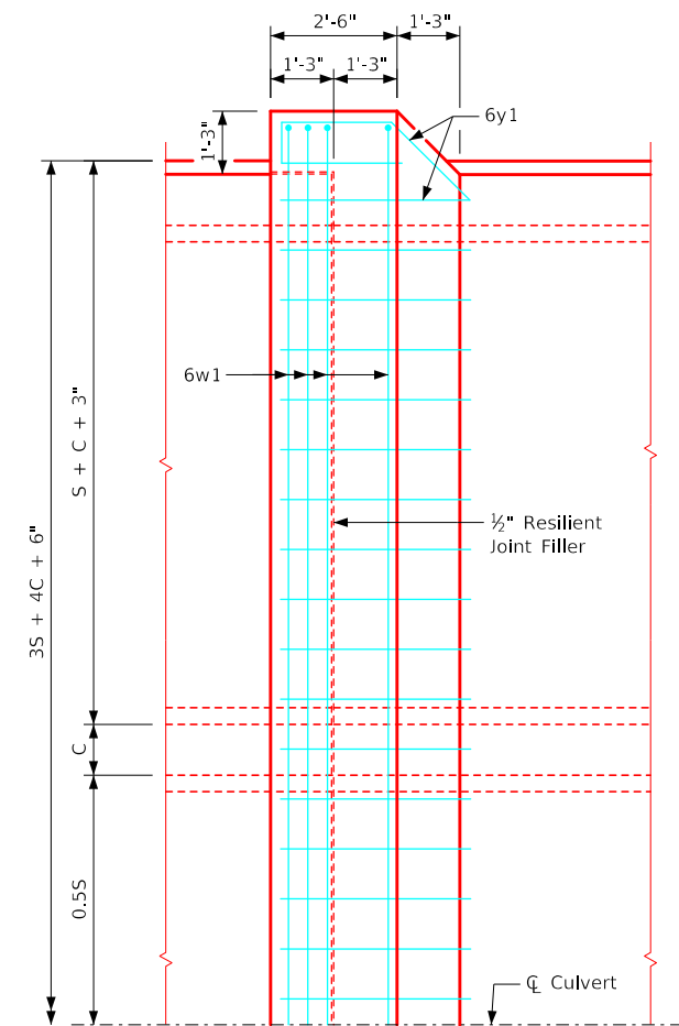
Plan View - Slab
