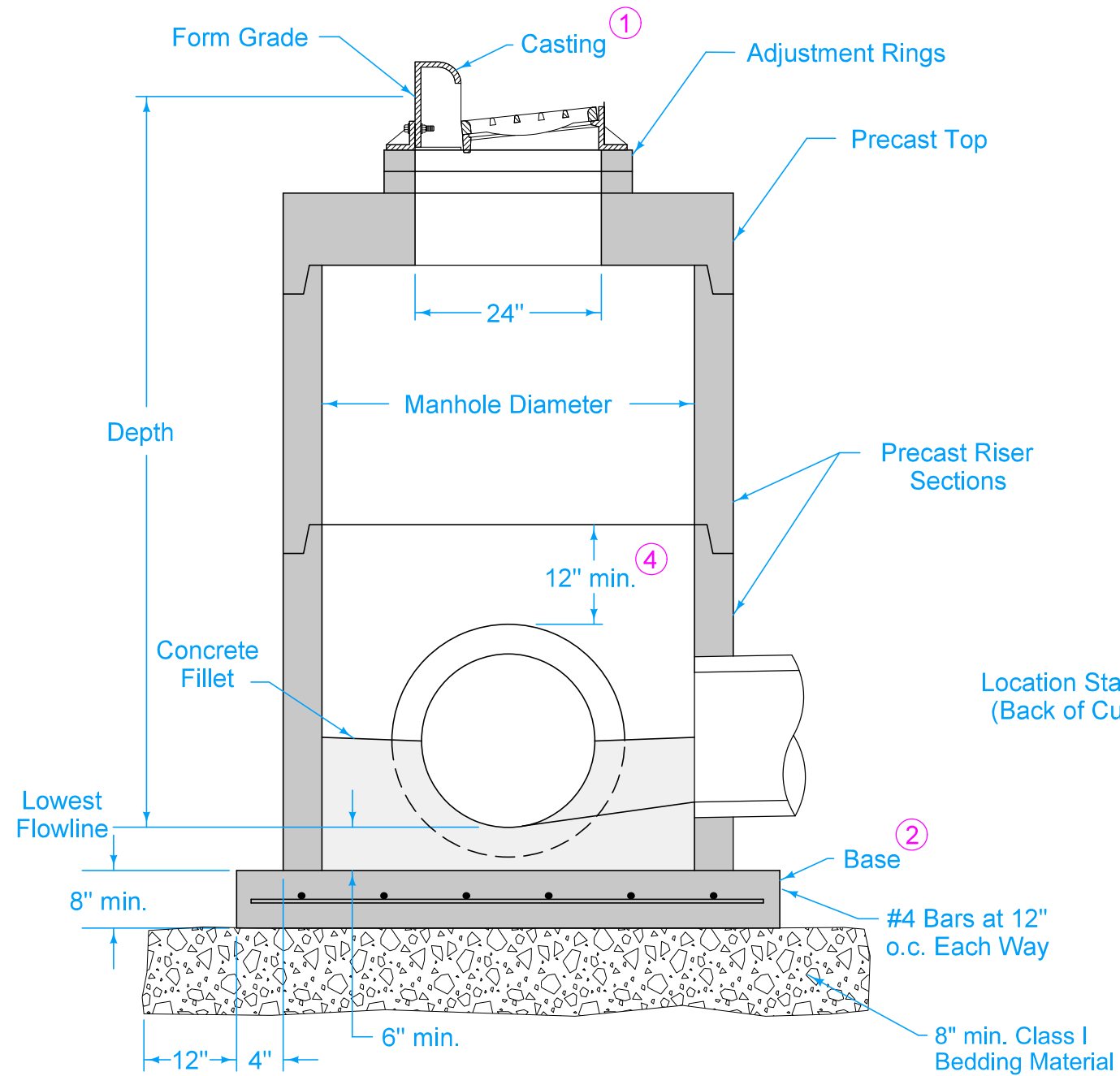
TYPICAL SECTION
