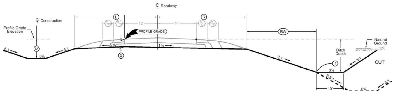
Figure 1: Typical cross section of a normal ditch.
