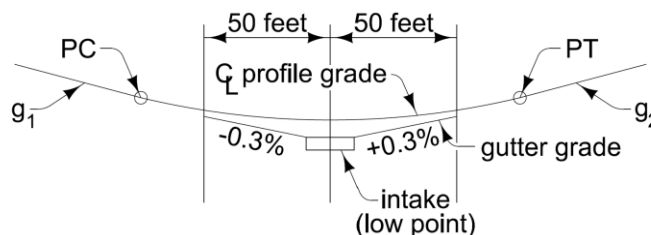
Figure 3: Sag vertical curve showing a minimum gutter grade.
