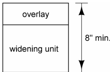
Figure 1: Minimum pavement widening thickness.
