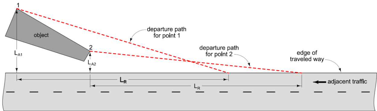
Figure 7: Departure paths for skewed or irregularly shaped objects.
