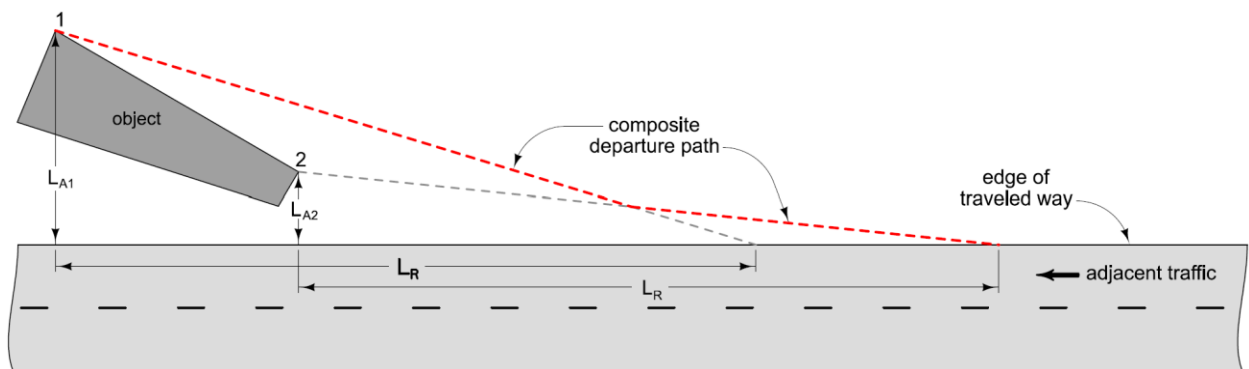
Figure 8: Defining a composite departure path.
