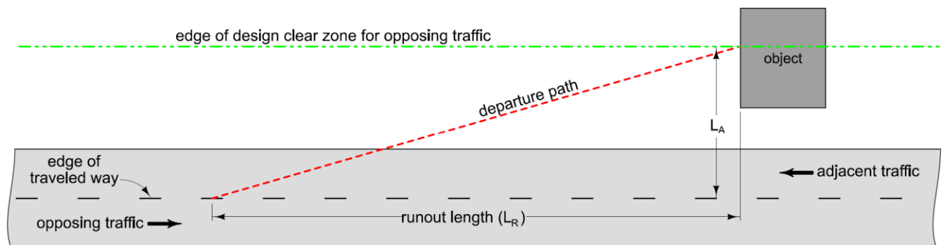
Figure 4: Departure path for opposing traffic.
