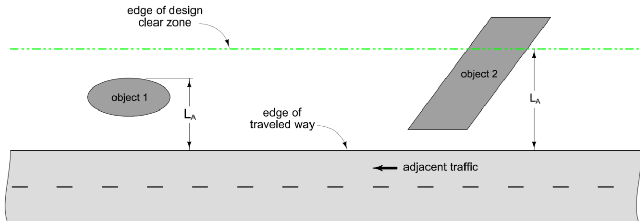
Figure 2: Comparison of L_A distances for different objects.
