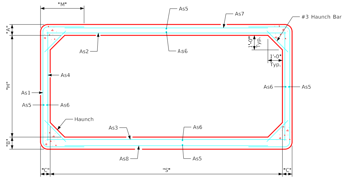
Typical Barrel Section
