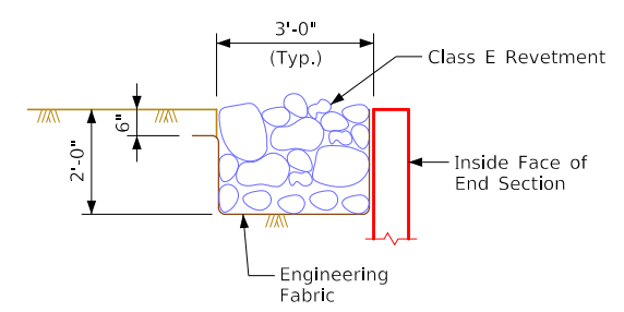
Section A-A Typical Details
