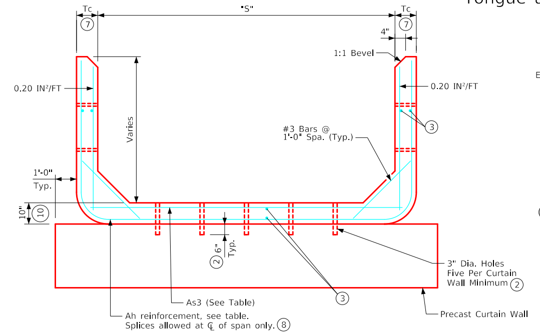
Section Z-Z
