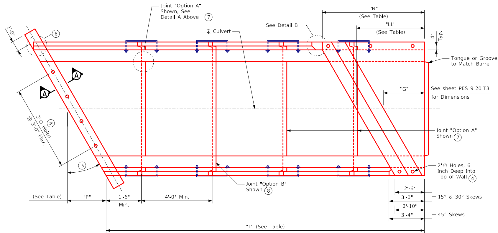
Plan View
