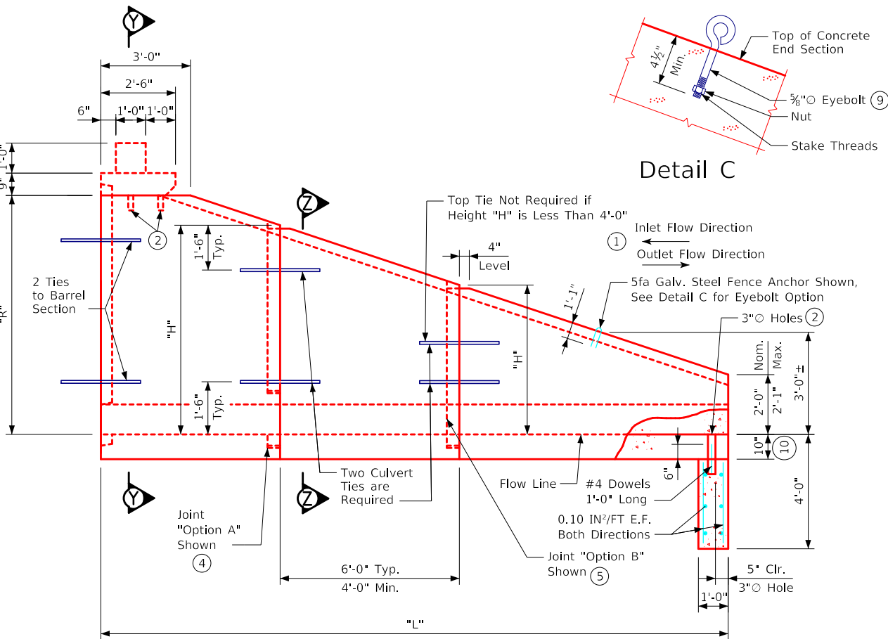
Side Elevation
